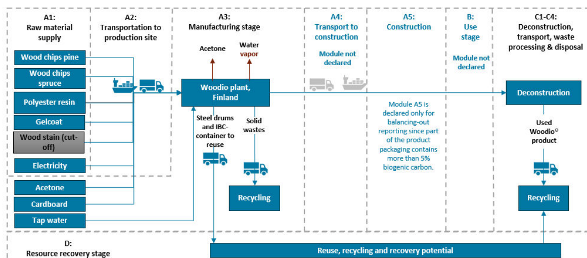
Figure 1. System diagram.
